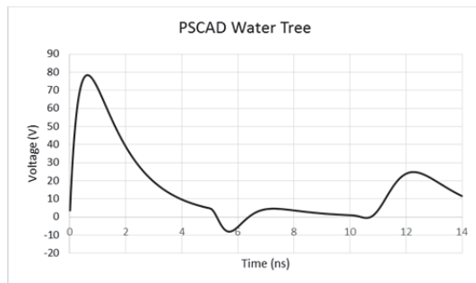
Figure 8: Input voltage in PSCAD simulation with water tree
