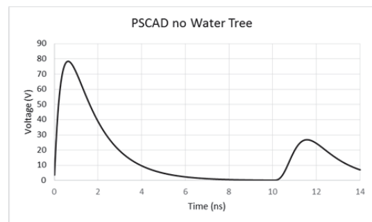
Figure 6: Input voltage in PSCAD simulation with no water tree
