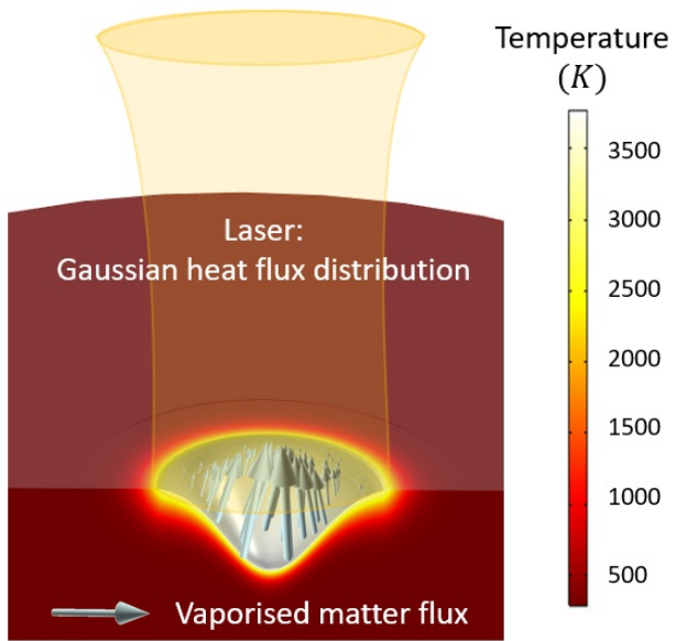
Figure 1: Laser beam heating material and crater creation by vaporisation.
